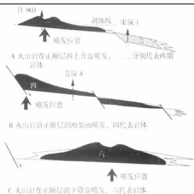
图 1 徐家围子断陷火山岩喷发- 赋存型式 Fig. 1 Eruption - occurrence patterns of volcanic rocks in Xujiaweizi fault- depression
